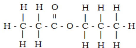
Propyl proanoate
