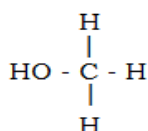
Methanol
