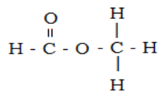
Methyl methanoate
