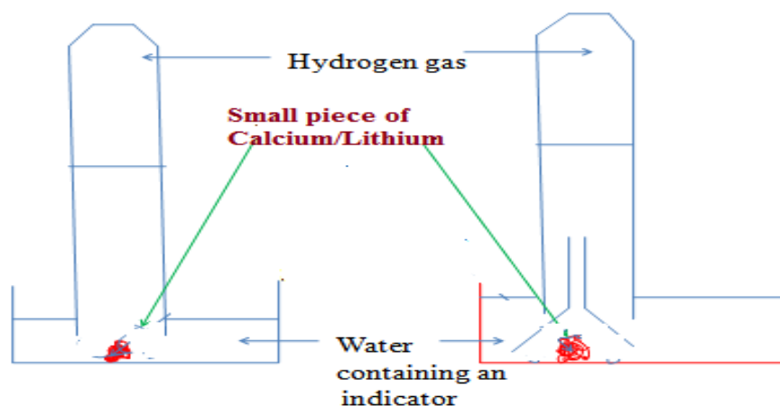
Collection of hydrogen from reaction of Lithium /calcium with water
