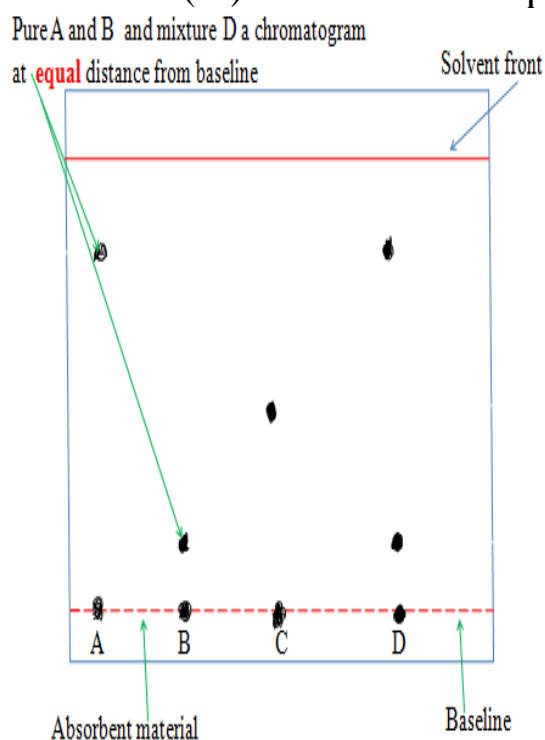
Chromatogram showing pure A,B,C and mixture D
