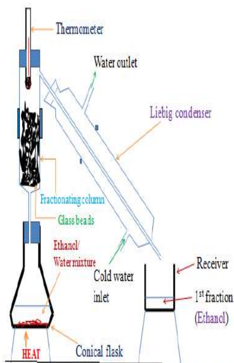
Fractional Distillation of miscible ethanol/water mixture
