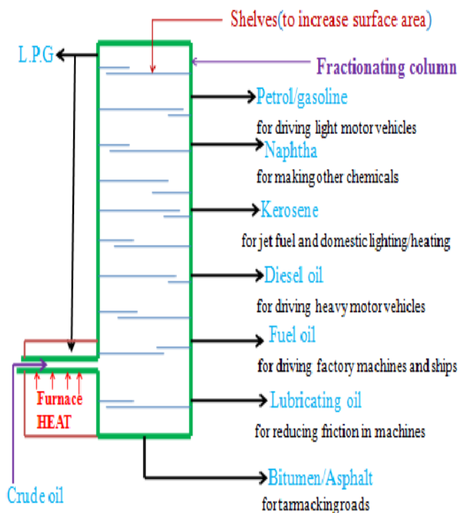
Industrial fractional distillation of crude oil in an oil refinery
